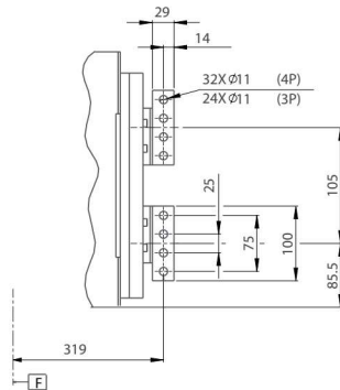
Rated Current 2900-3200A
