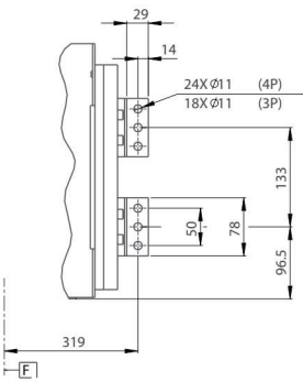
Rated Current 2000-2500A
